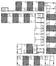
3 rd - 5 th FLOOR PLAN
